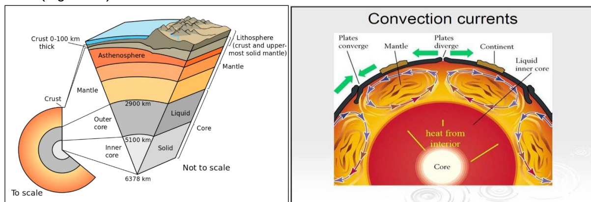
Figure 1- a) Figure showing the zoned internal structure of the Earth b) Schematic view of convection currents resulting from the movement of magma
